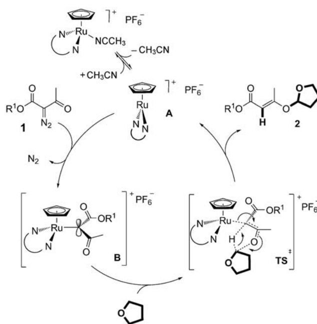
Scheme 2. Mechanistic rationale. NN corresponds to 1,10-phenantroline ( L1 ).
